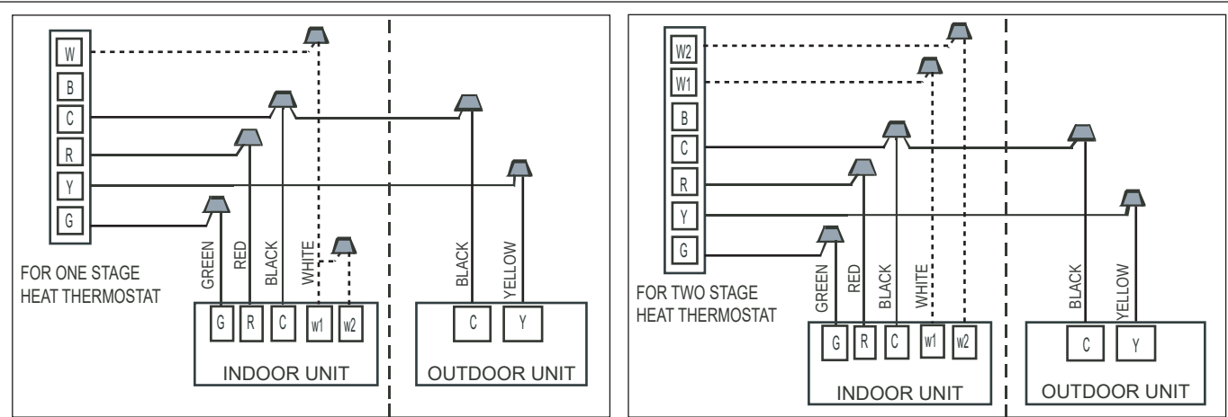
Control Wiring for A/C Systems
