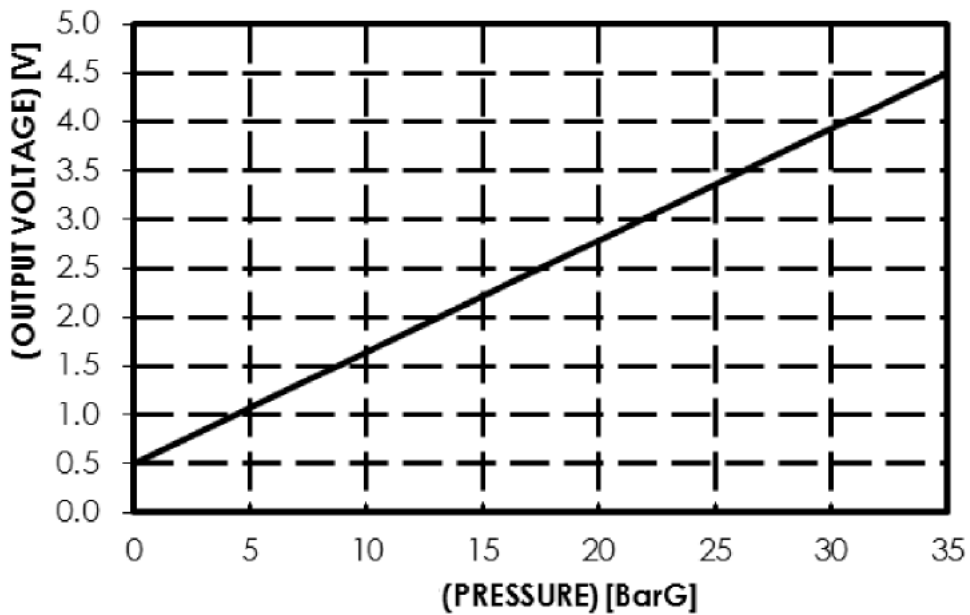
Pressure sensor Figure 1 (OUTPUT CHARACTERISTICS)
