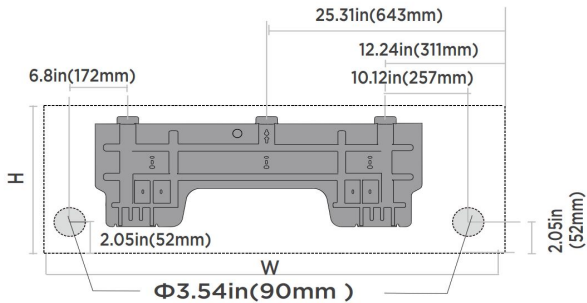
Indoor unit dimensions(WxH): 49.57in(1259mm)x14.25in(362mm)
