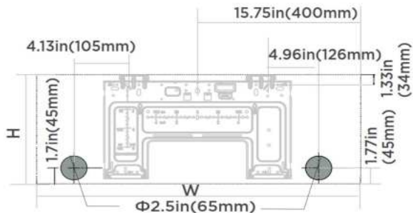
Indoor unit dimensions(WxH): 28.7in(729mm)x11.5in(293mm)
