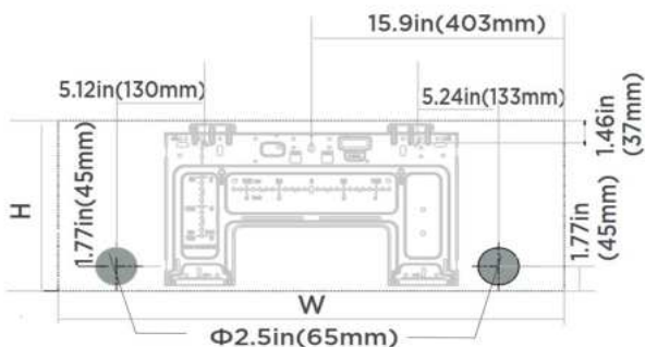
Indoor unit dimensions(WxH): 31.7in(806mm)x11.65in(296mm)
